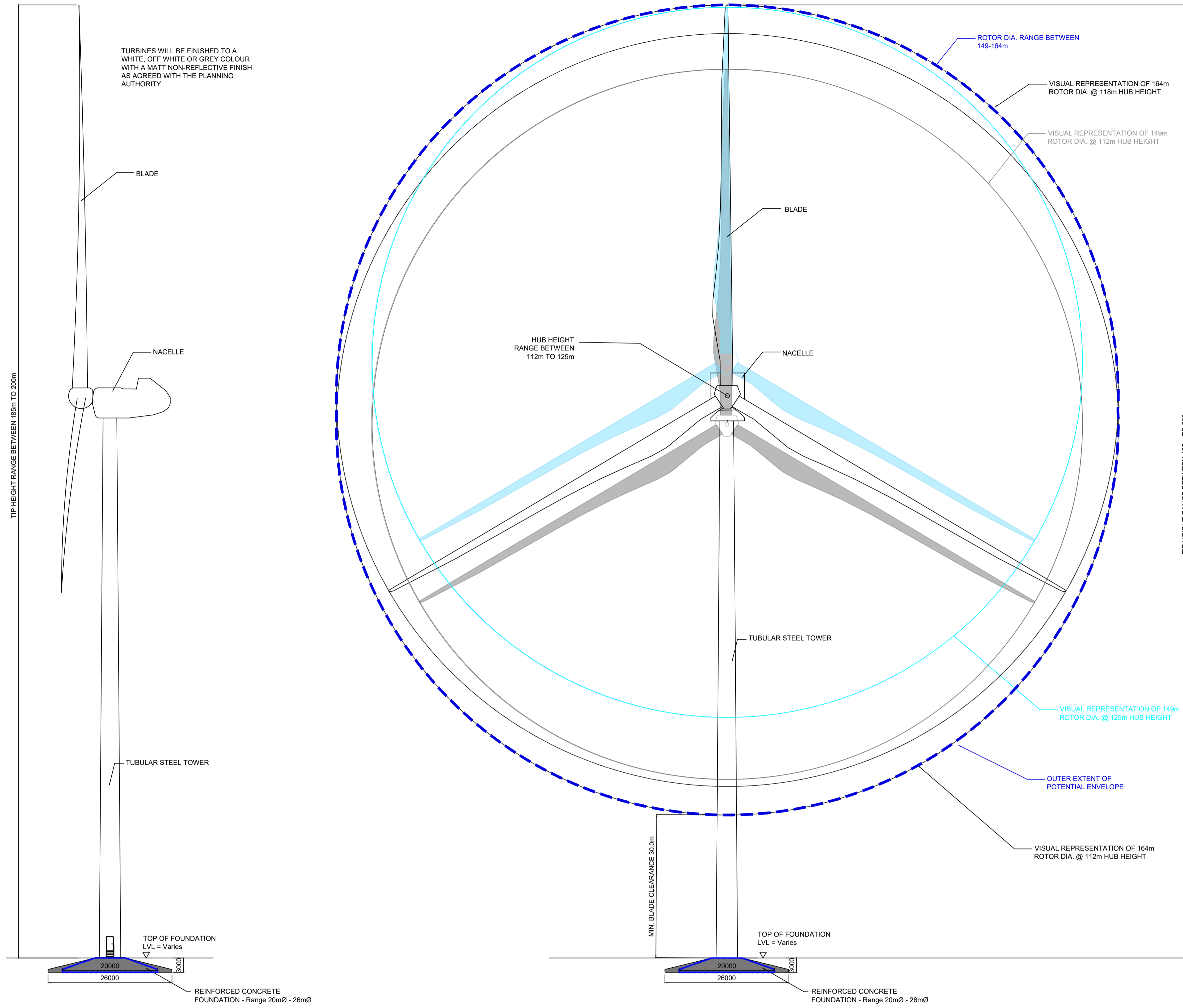
TYPICAL TURBINE SIDE ELEVATION
