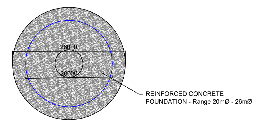
TYPICAL TURBINE FOUNDATION PLAN
